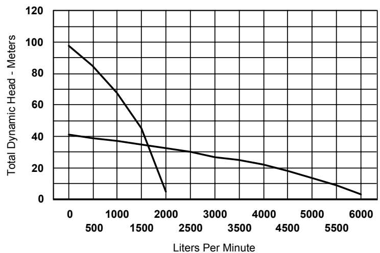
Piranha pump model P3000, HV & HH 22.4 kw, 50 hz
