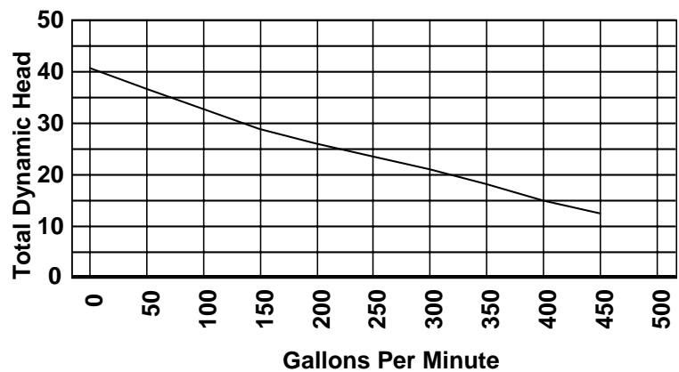
Piranha Solids Handling Pump Model PLS 300
