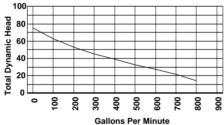
Piranha Solids Handling Pump Model PLS 750
