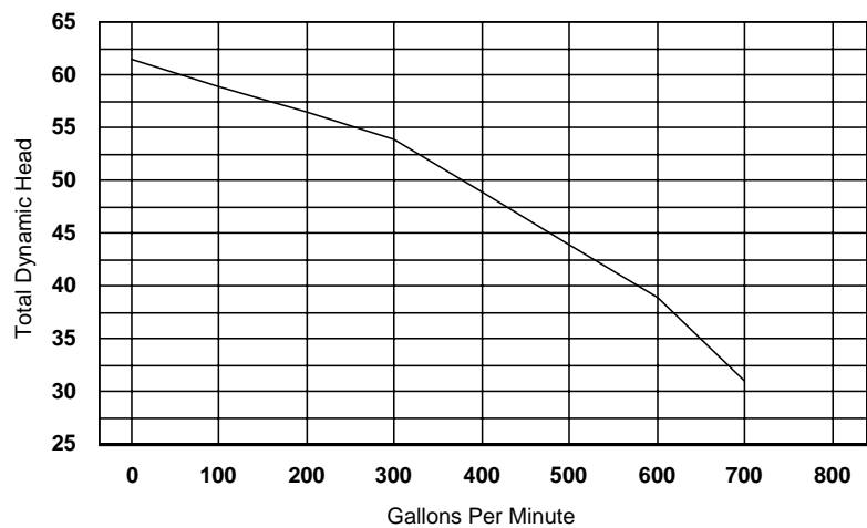
Piranha Agitator/Slurry Pump Model PS-1500-A
