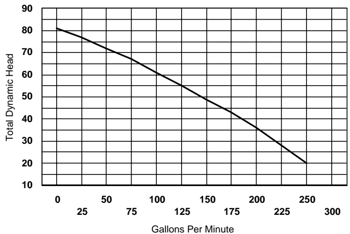
Piranha pump model PSS-500 5 hp, 460v, 3 phase
