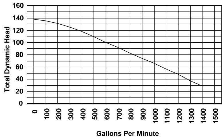
Piranha Solids Handling Pump Model PLS 3000
