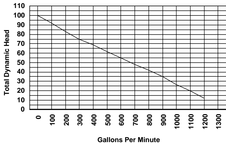
Piranha Solids Handling Pump Model PLS 1500
