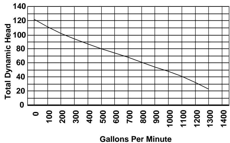
Piranha Solids Handling Pump Model PLS 2000
